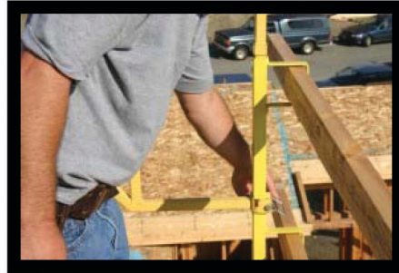
Slide End Gate into handrail and pin in place.
